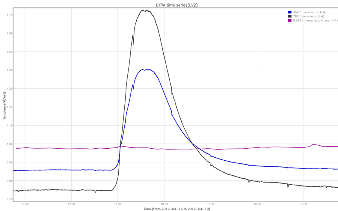
M1.7 Flare - East limb, 16/04 at 17:49 - LYRA curves
