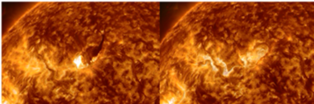
C8.7-flare at 00:30UT
