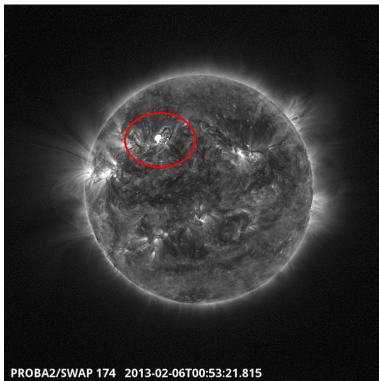
C8.7 flare on 6 February
