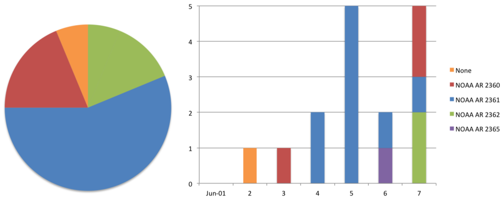
Distribution of >B flares, June 1 – 7, 2015
