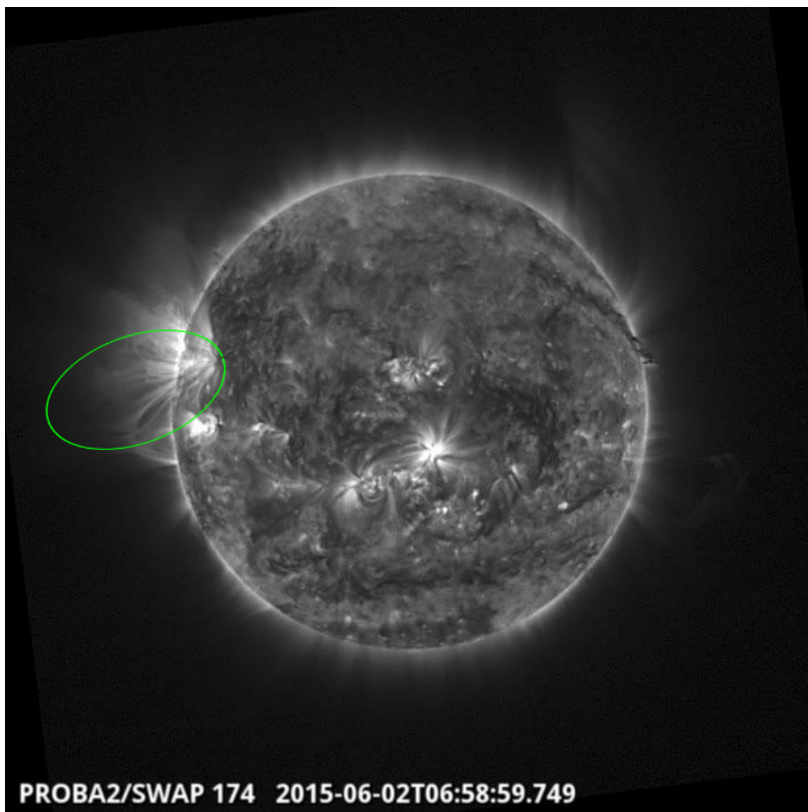
Eruption on the east limb @ 06:58 SWAP image Find a movie of the events here (SWAP movie) http://proba2.oma.be/swap/data/mpg/movies/20150602_swap_movie.mp4
