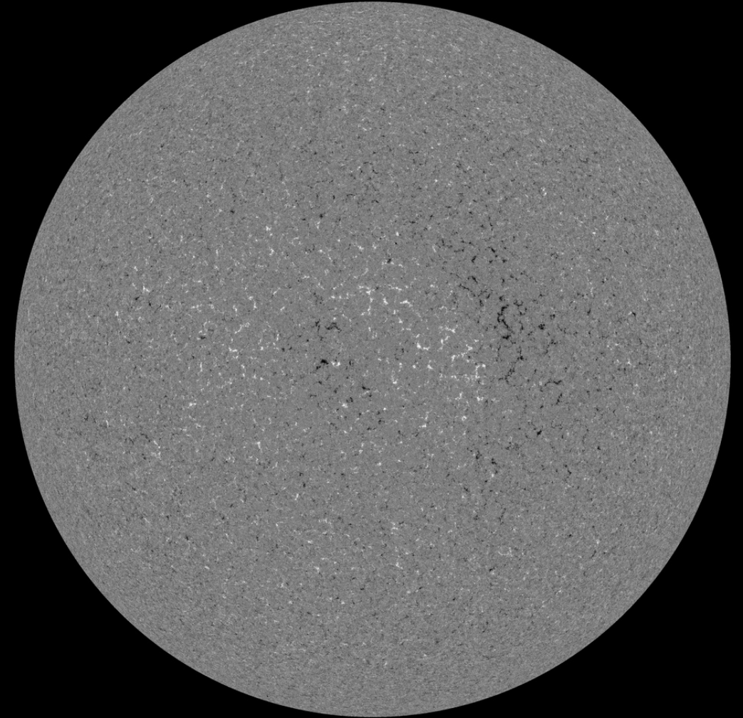
SDO/HMI Magnetogram 2019-07-31
