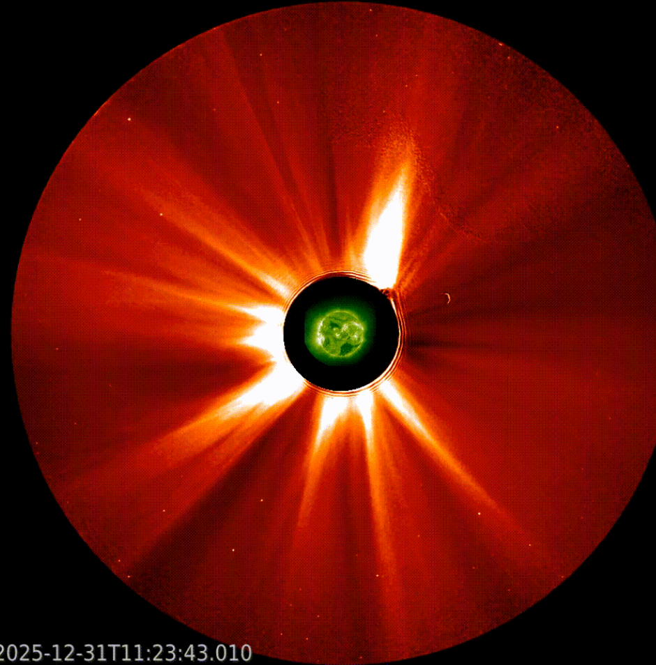
STEREO-A/COR2
