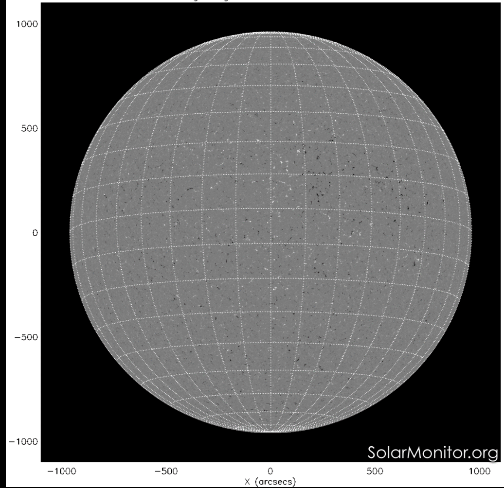
SDO HMI Magnetogram 25-Mar-2018 10:46:36.700
