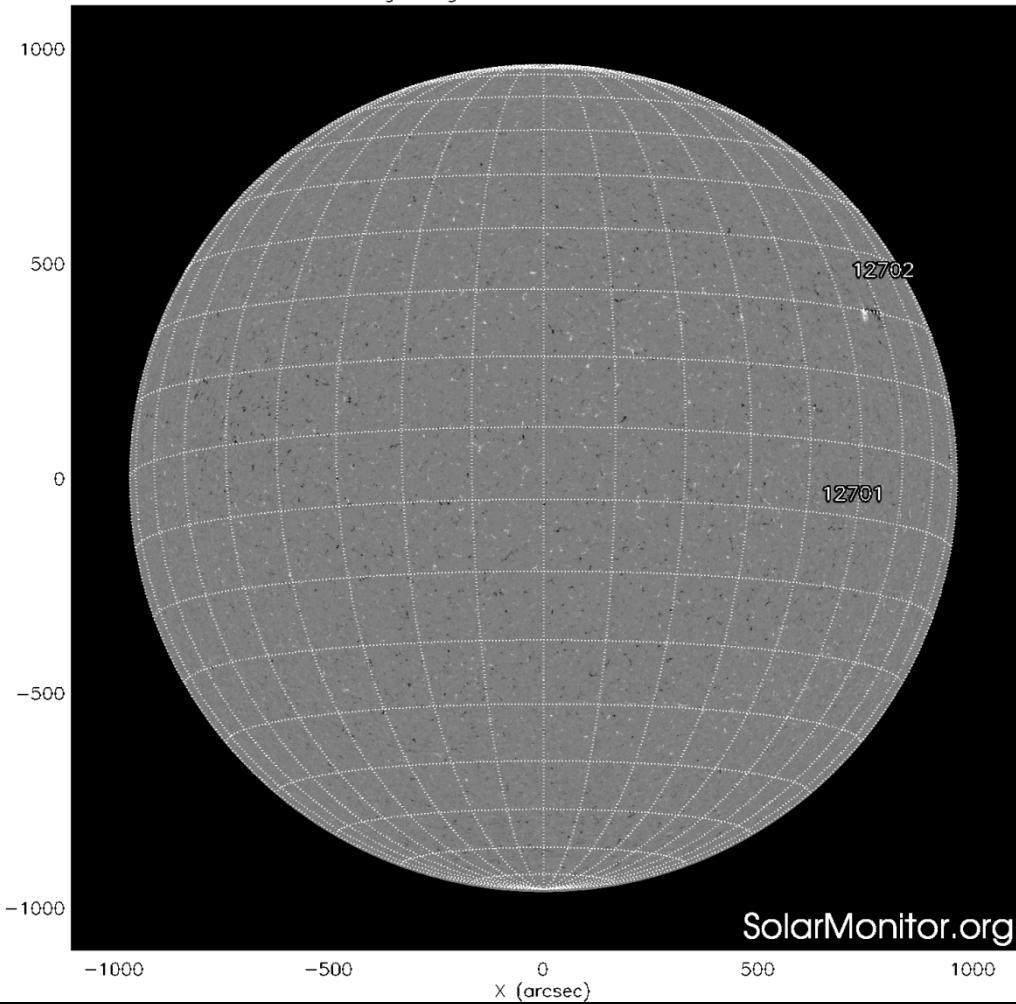
SDO HMI Magnetogram 18-Mar-2018 19:46:35.600
