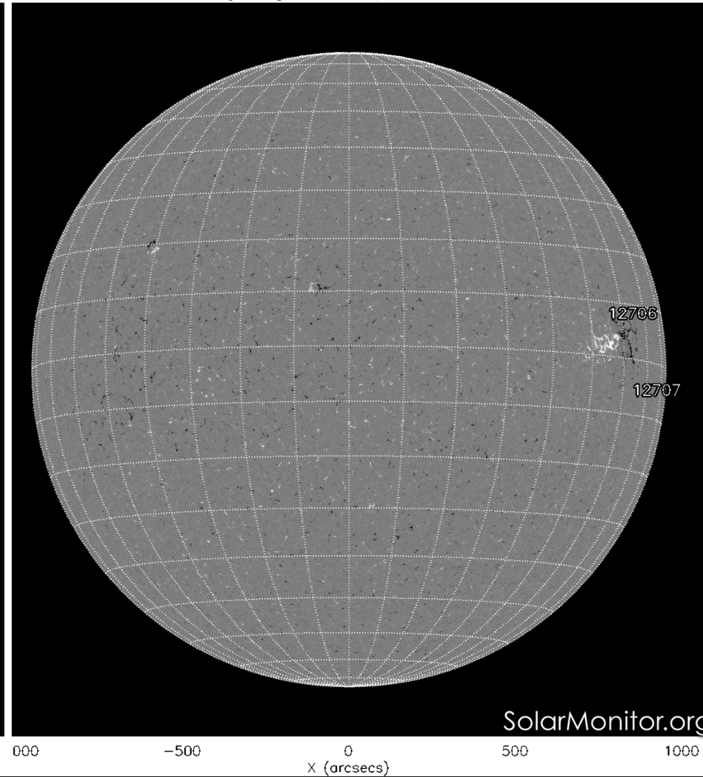
SDO HMI Magnetogram 29-Apr-2018 14:34:41.500
