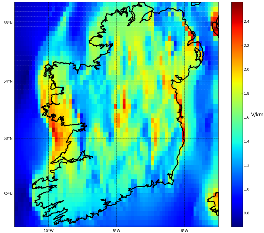
Calculated E-Field for March 1989 Storm
