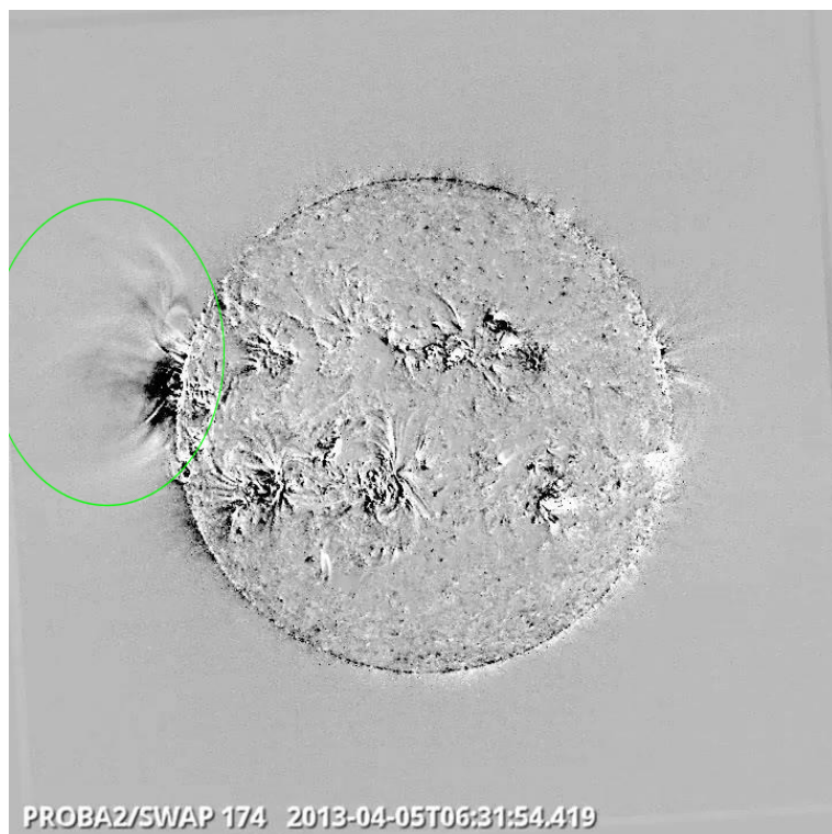
C2.1 flare near the east limb @ 06:31UT - SWAP difference image
