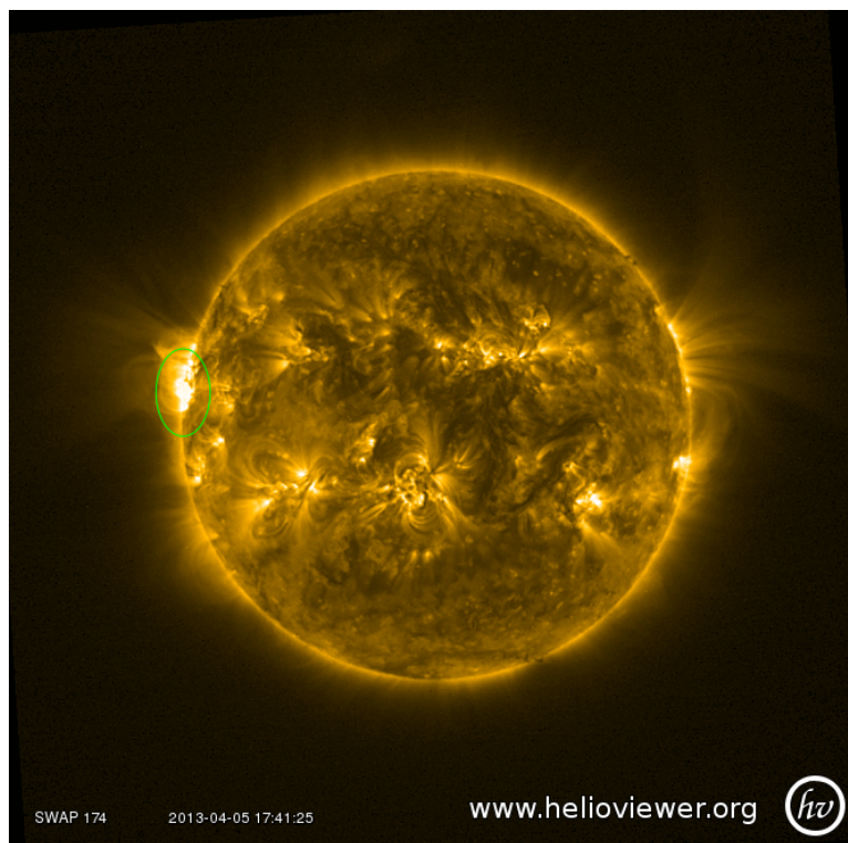
M2.2 flare on the east limb @ 17:41UT - SWAP image, colored, from HelioViewer.org.
