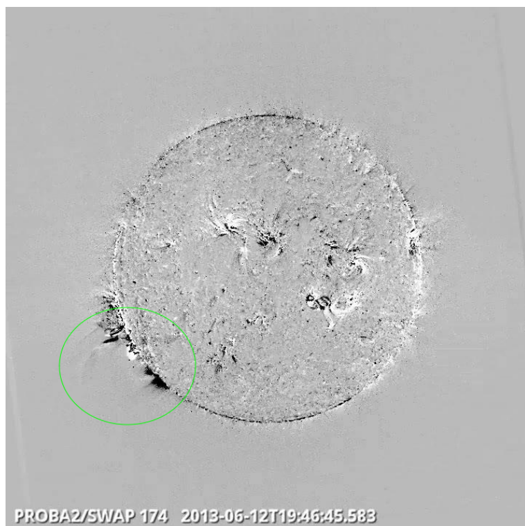
B4.4 flare + Prominence Eruption South West limb @ 19:46 - SWAP difference image
